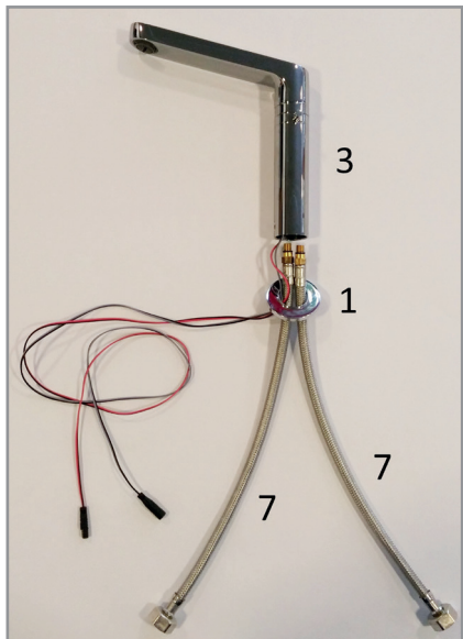
Step A – Mounting flex hoses and ring
