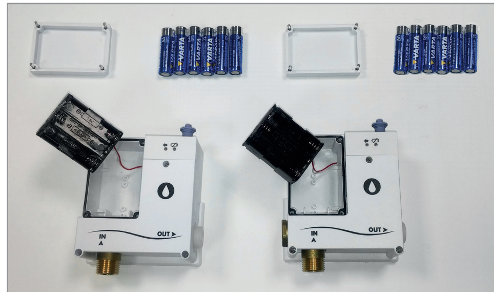
Step D – Assembling 12xAA batteries (not included)
