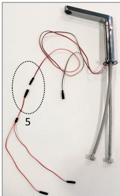
Step B – Connecting Y cable
