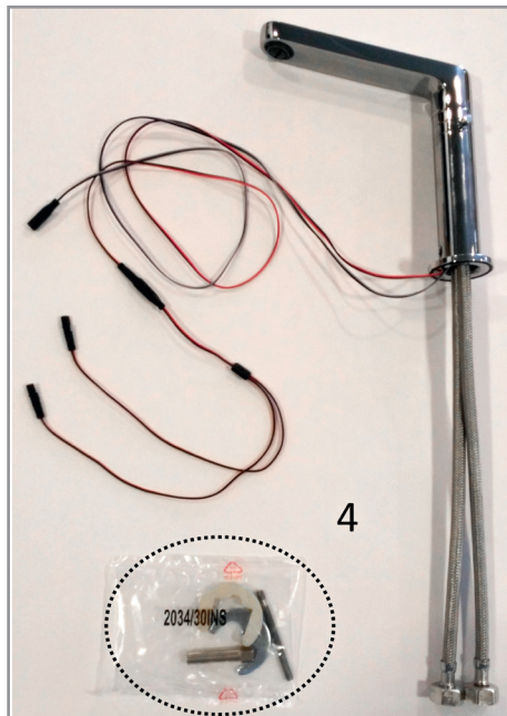
Step C – Fixing the mixer
